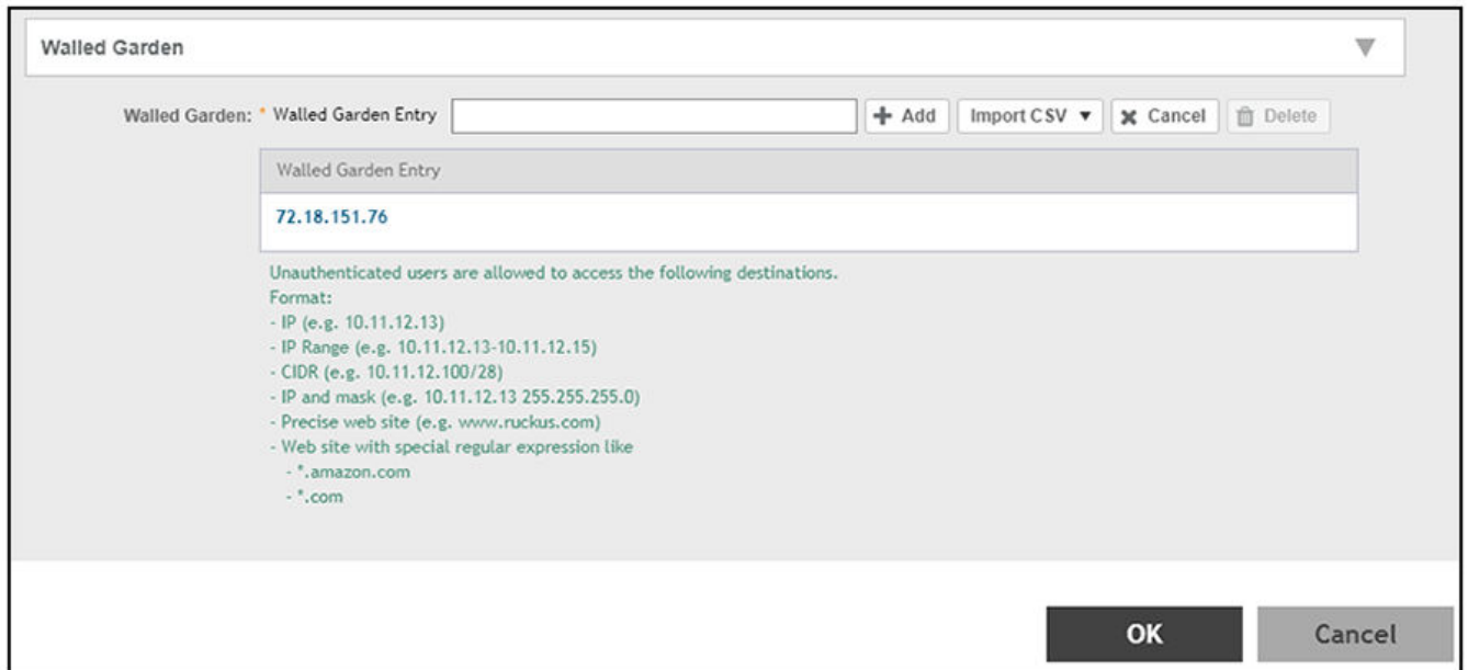
FIGURE 107 Walled Garden Configuration for SmartZone
