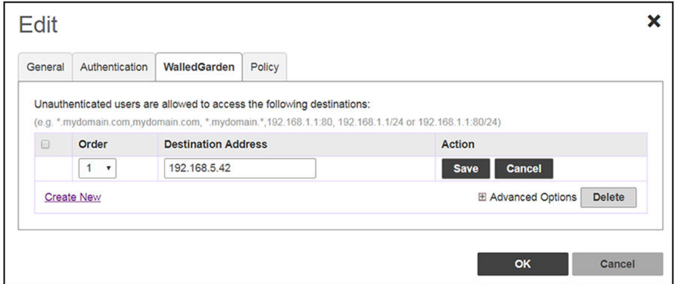
FIGURE 108 Walled Garden Configuration for Unleashed
