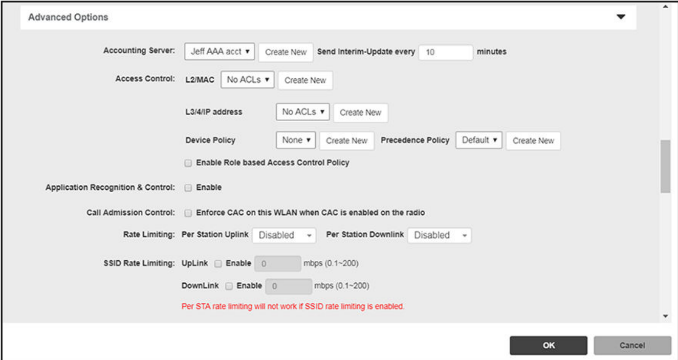
FIGURE 116 Select RADIUS Accounting Server on ZoneDirector
