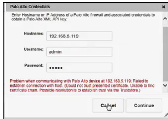
FIGURE 125 Possible Error Message While Cloudpath Tries to Connect to Palo Alto Firewall
