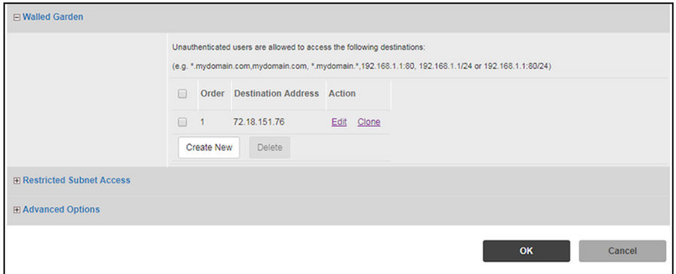
FIGURE 107 Walled Garden Configuration for SmartZone
