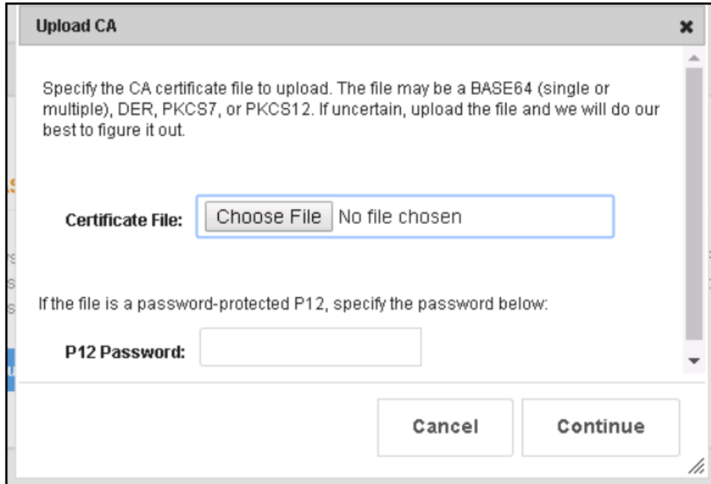
FIGURE 122 Truststore Upload Popup to Add New Certificate
