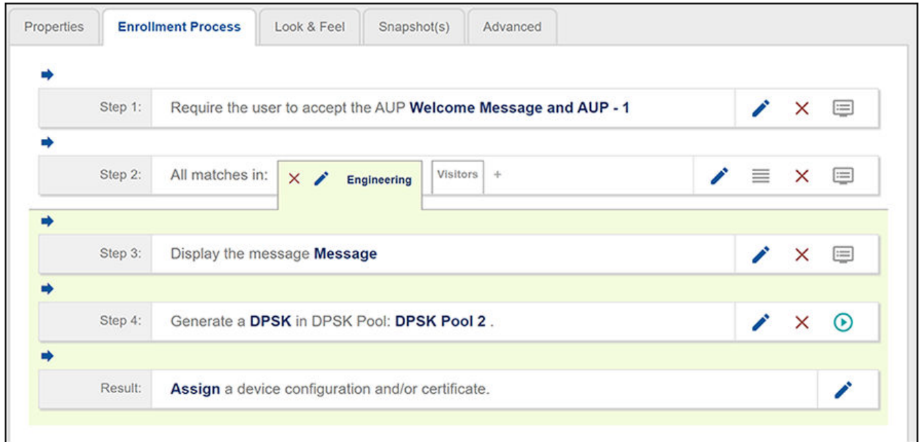
FIGURE 90 Workflow Split Example
