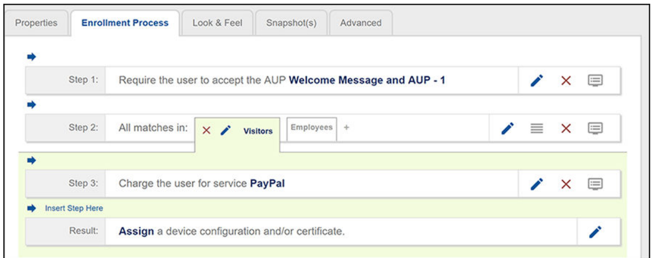
FIGURE 72 Workflow After Adding PayPal "Charge User for Service" Step
